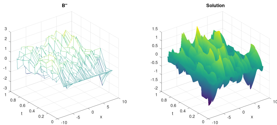
Figure 2: H_0 = H_1 = \frac{1}{4}
