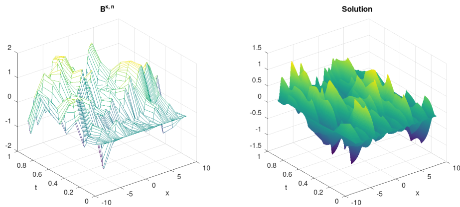
Figure 1: H_0 = H_1 = \frac{1}{4}
