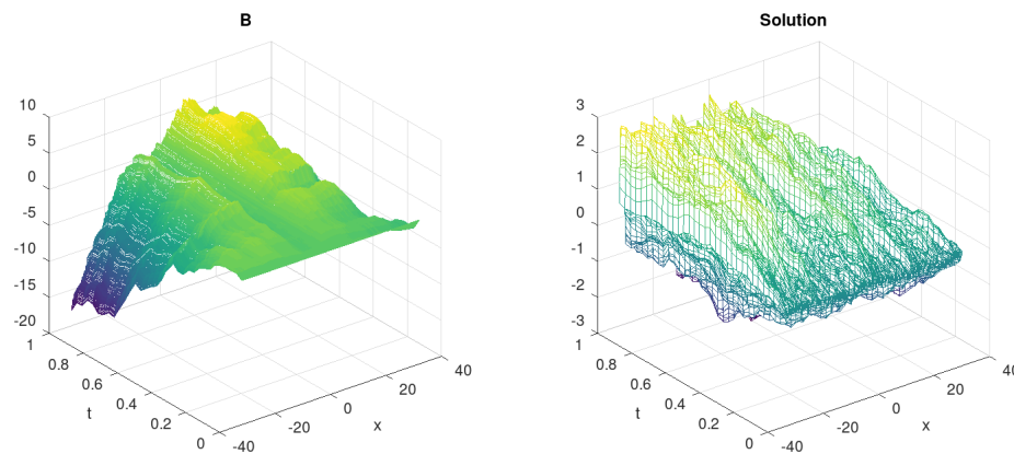
Figure 4: H_0 = H_1 = \frac{3}{4}
