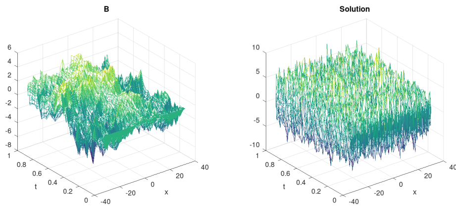
Figure 3: H_0 = H_1 = \frac{1}{4}
